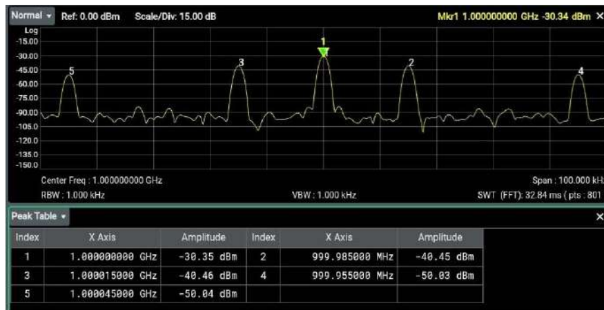
Figure 5.13 Peak Table
