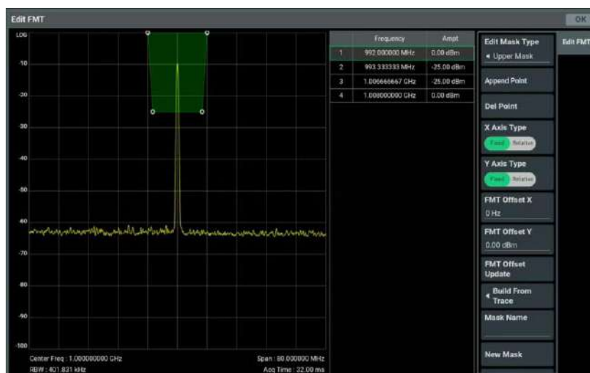
Figure 6.8 FMT Editing Interface
