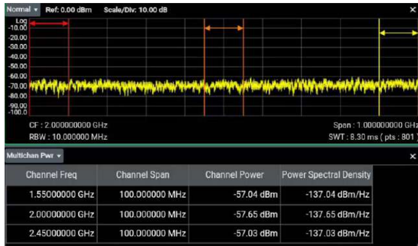
Figure 5.5 Channel Power Measurement Interface
