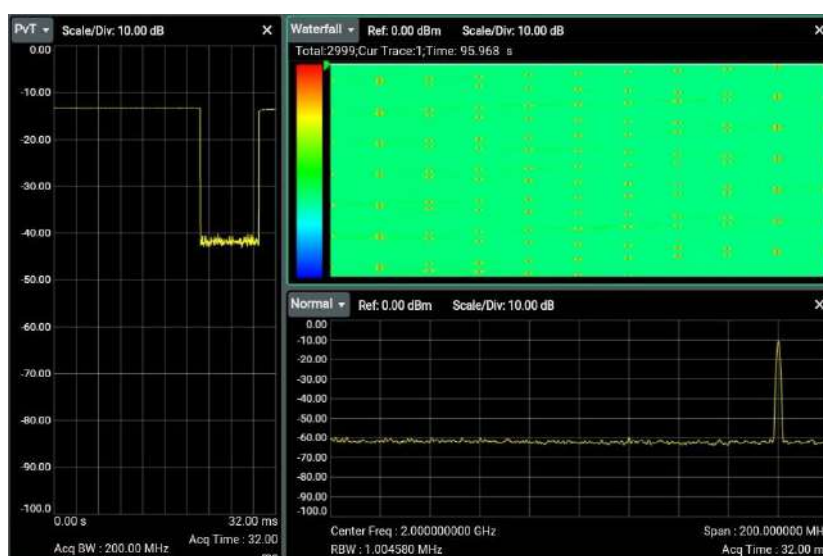
Figure 6.7 PvT/Normal/Waterfall Plot View
