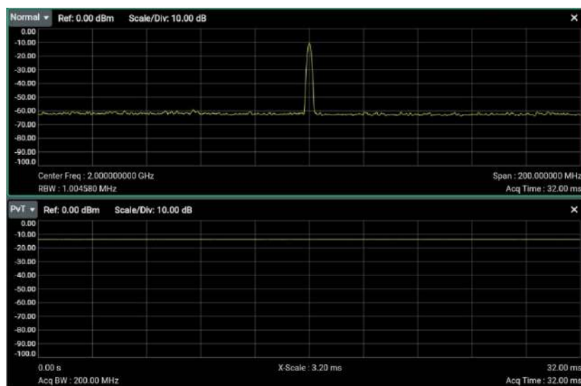
Figure 6.6 PvT/Normal View
