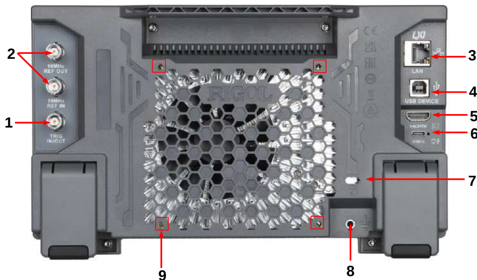
Figure 4.6 Rear Panel of DNA800 Series
