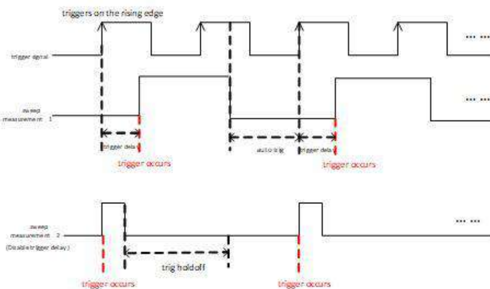
Figure 5.1 Relationship of Trigger Parameters
