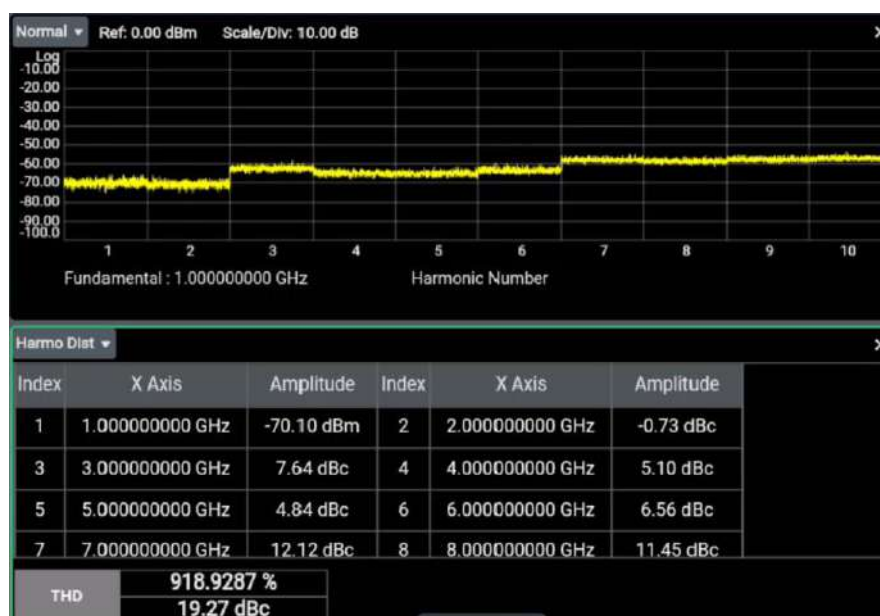
Figure 5.7 Harmonic Distortion Measurement Interface
