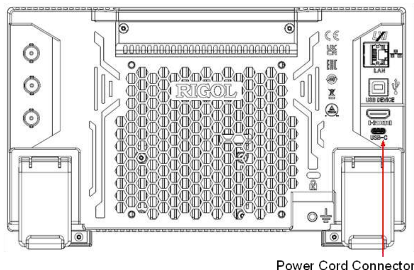
Figure 4.4 To Connect to AC Power
