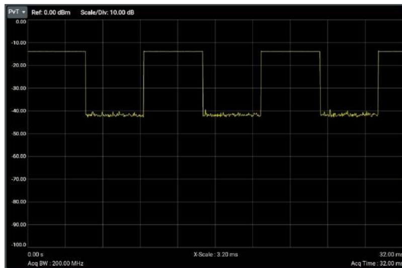
Figure 6.5 PvT View
