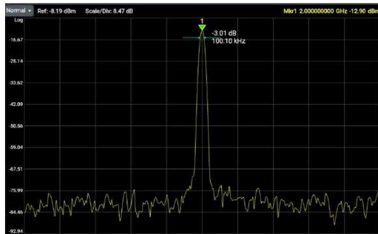
Figure 5.12 N dB Bandwidth Measurement
