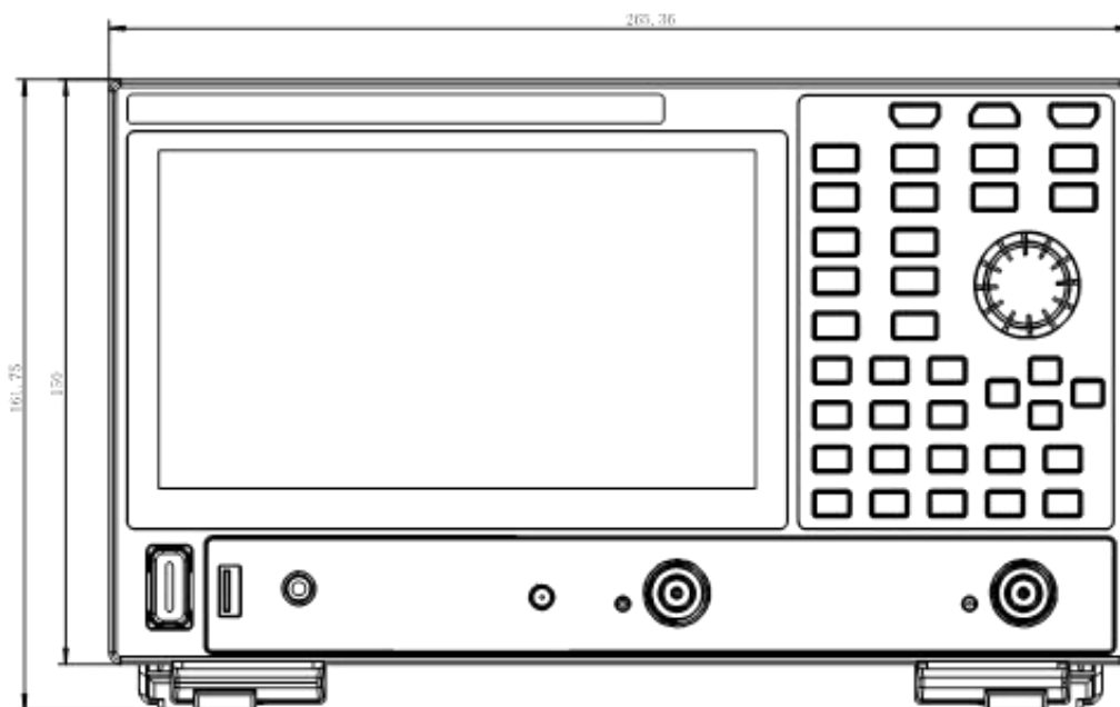
Figure 4.1 Front view (mm)
