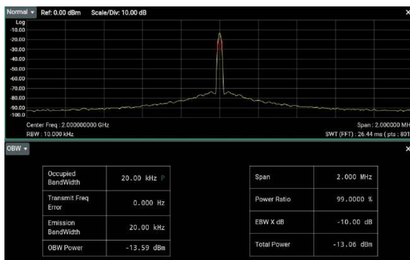
Figure 5.8 OBW Measurement Interface
