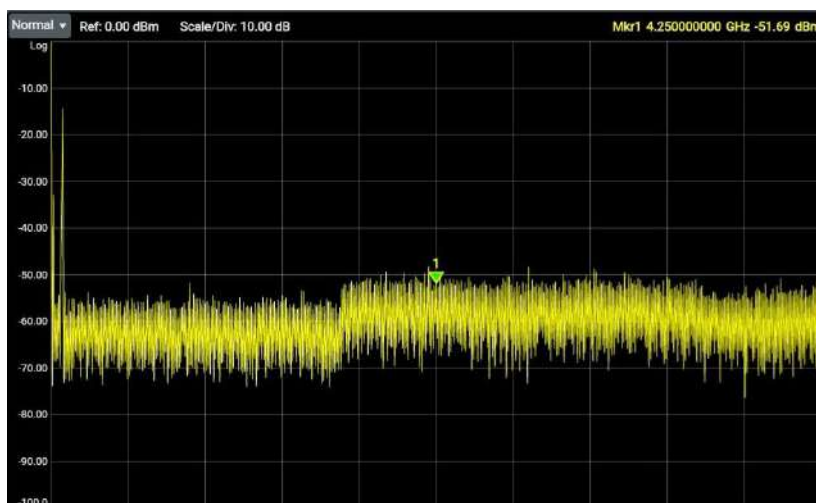
Figure 5.10 Marker
