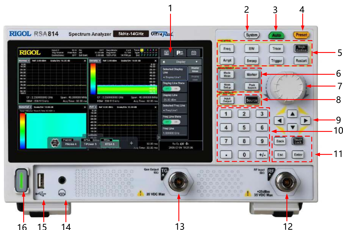
Figure 4.5 RSA800 Series Front Panel
