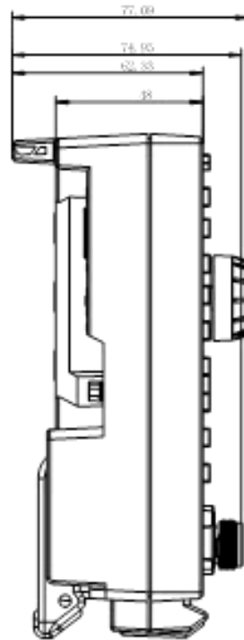
Figure 4.2 Side view (mm)
