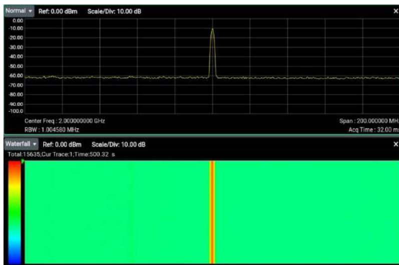
Figure 6.2 Spectrogram View
