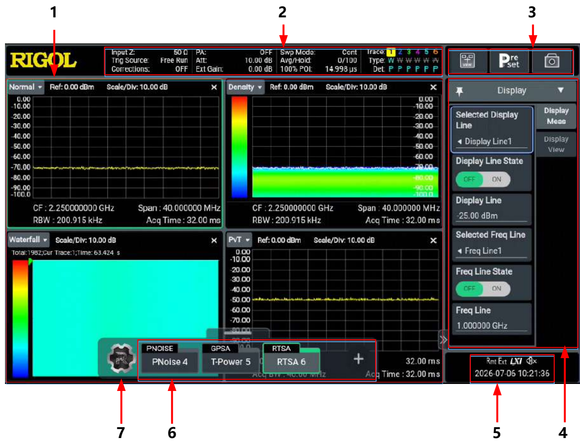
Figure 4.7 User Interface
