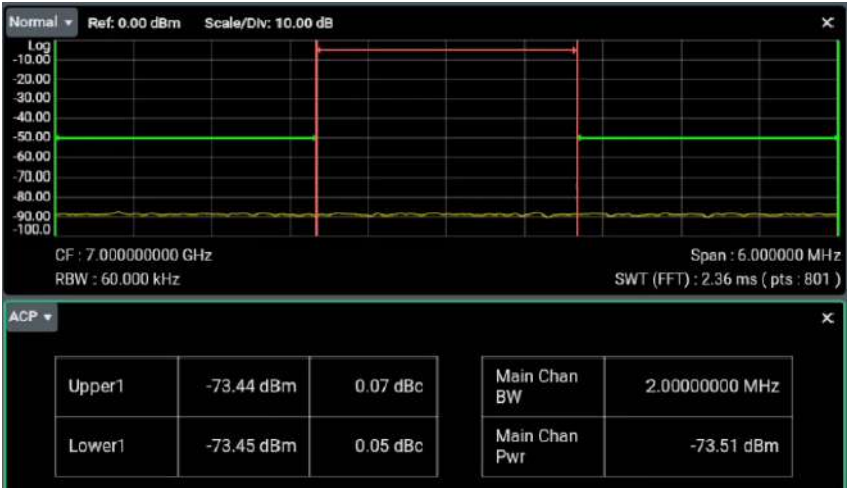
Figure 5.3 ACP Measurement Interface
