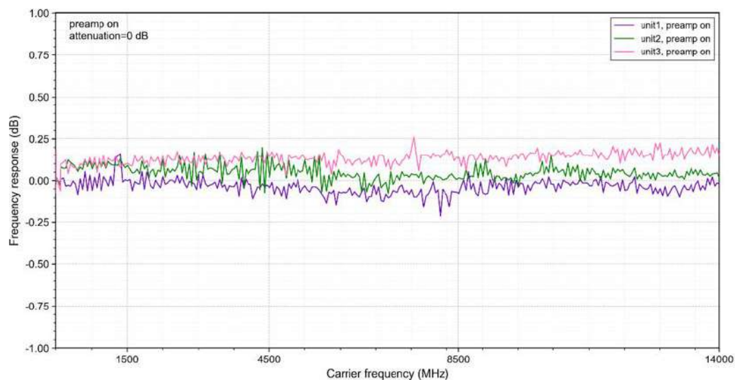
Frequency Response (attenuation = 0 dB, PA on)
