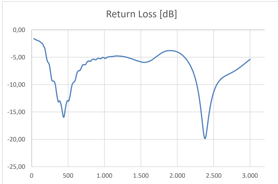
TBMA1B, S11, 30 MHz ... 3000 MHz
