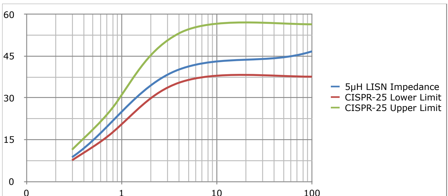
Picture 1 – 300kHz...100MHz, measured impedance of the 5 \mu H LISN
