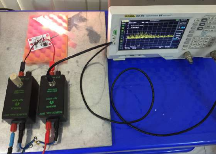
Picture 12 – Example: conducted emissions, pre-compliance measurement of an automotive LED driver using two LISNs
