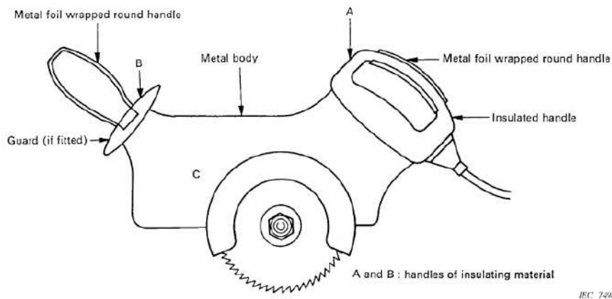
Figure 114 – Example from CISPR 16, portable electric saw with artificial hand
