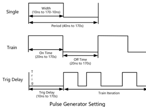
Pulse modulation; on/off ratio up to 80 dB
