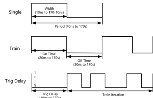
Pulse Generator Setting
