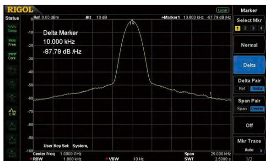
Phase noise < -98 dBc/Hz@10 kHz offset (DSA832/875)
