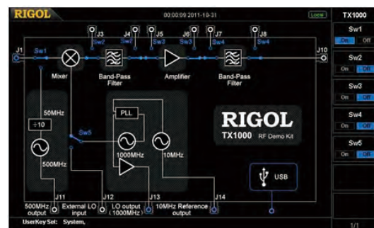
Built-in TX1000 panel control
