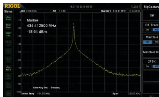
Capture ASK signal with the SSC kit
