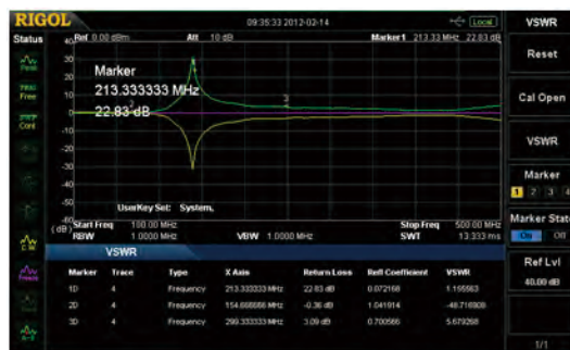
VSWR Measurement kit
