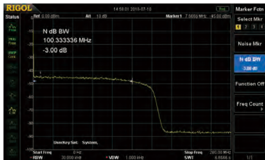
100 MHz bandwidth white Gaussian noise
