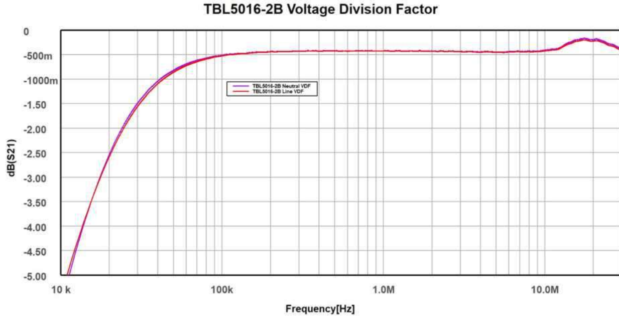
Voltage Division Ratio versus frequency, typ.
