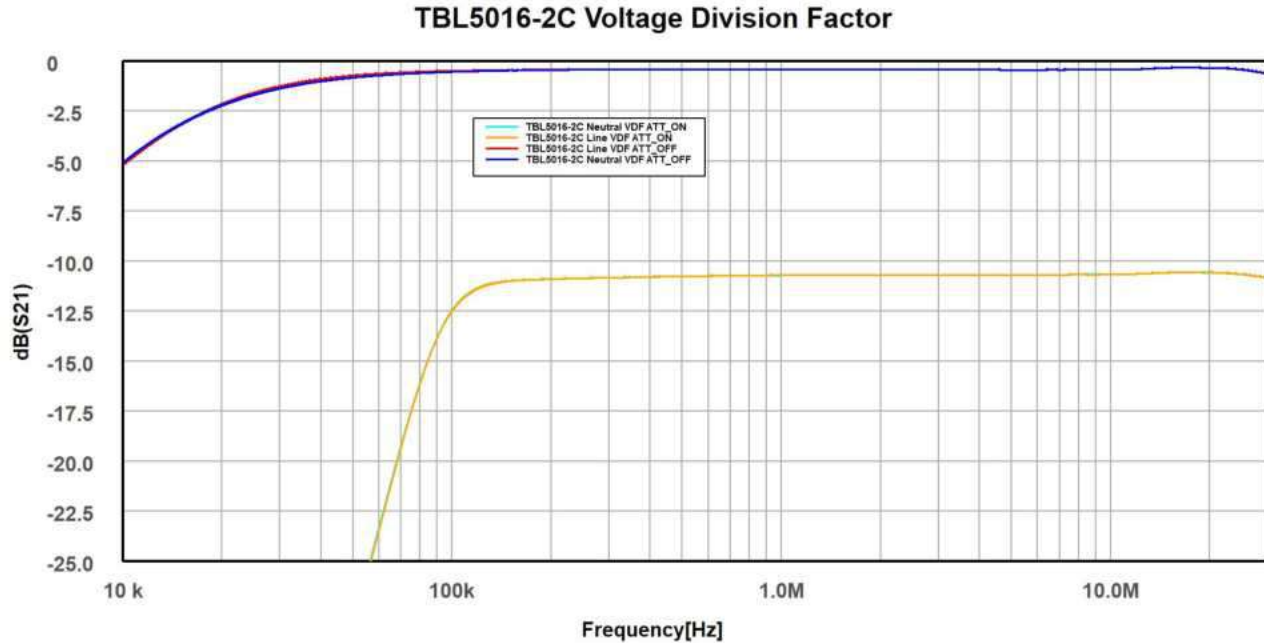
Voltage Division Ratio versus frequency, for Attenuator / Limiter / HPF “ON” and “OFF”
