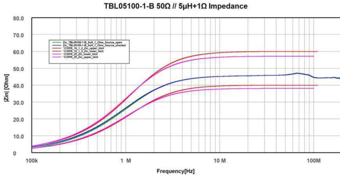
Picture 3: LISN impedance, 100 kHz – 110MHz; 50 \Omega // 5 \mu H+1 \Omega ; Jumper J1 open, Jumper J2 shorted
