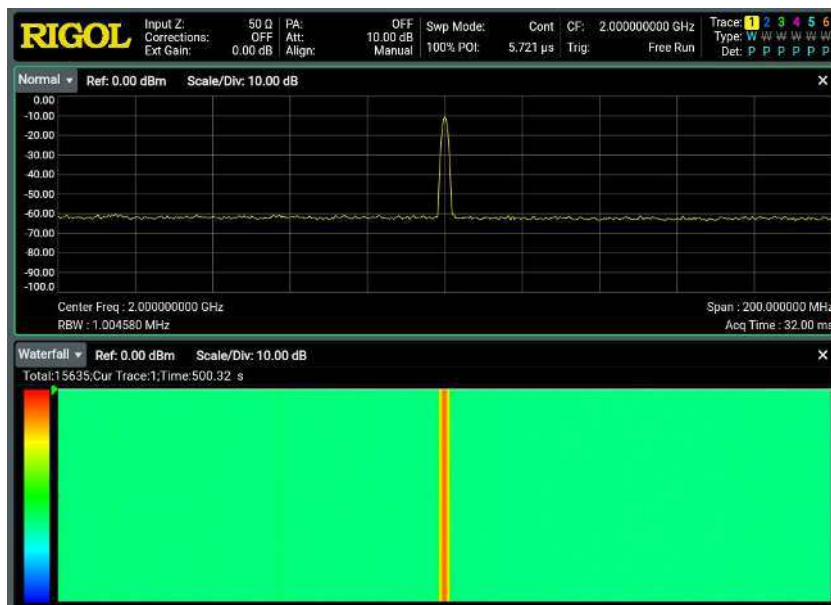
Figure 6.2 Spectrogram View
