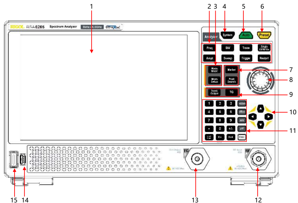
Figure 4.4 Front Panel
