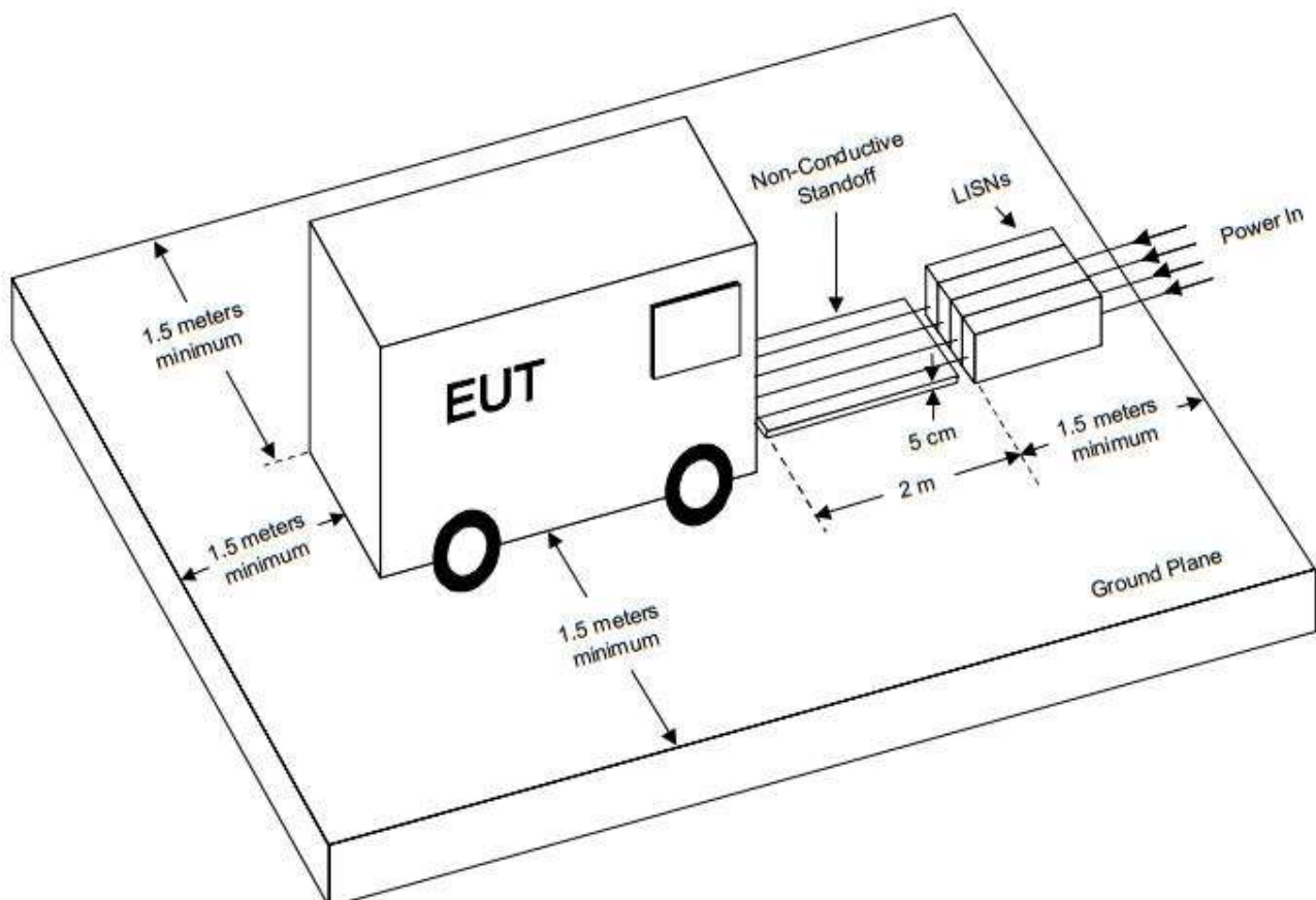
MIL-STD-461F test setup for free standing EUT
