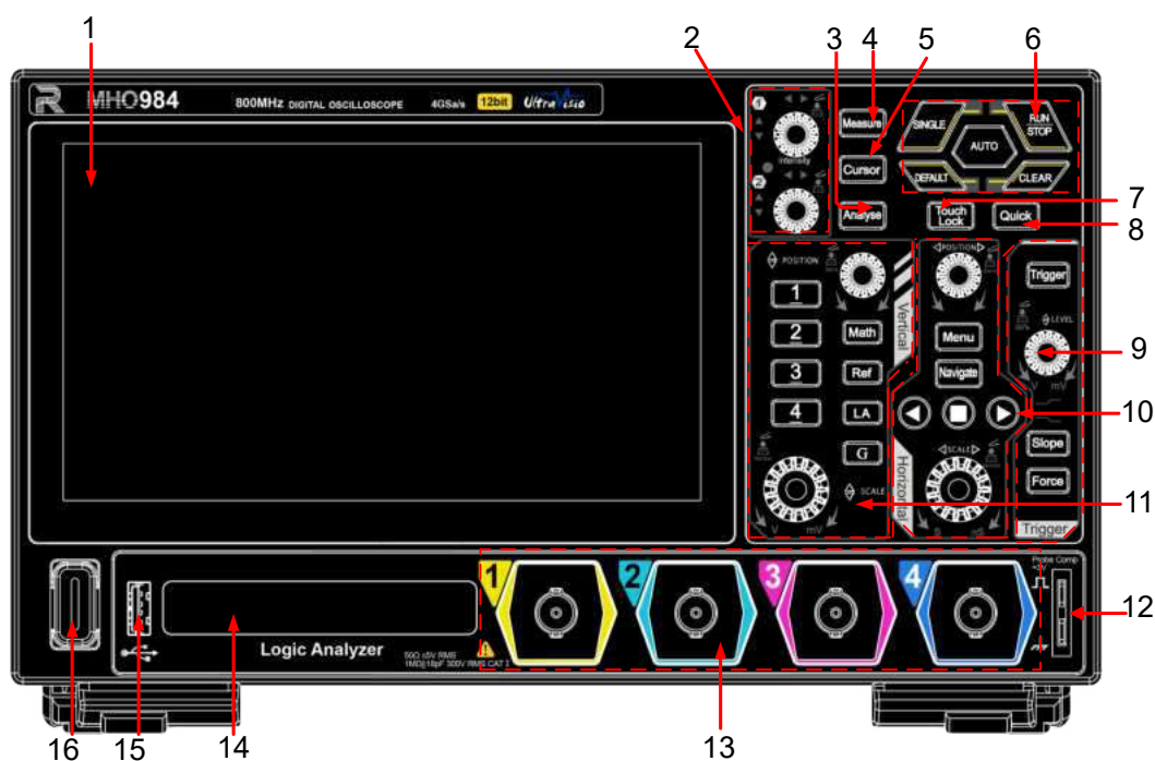
Figure 4.3 Front Panel
