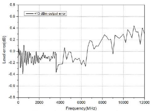
Measured at +13 dBm, level error vs frequency
