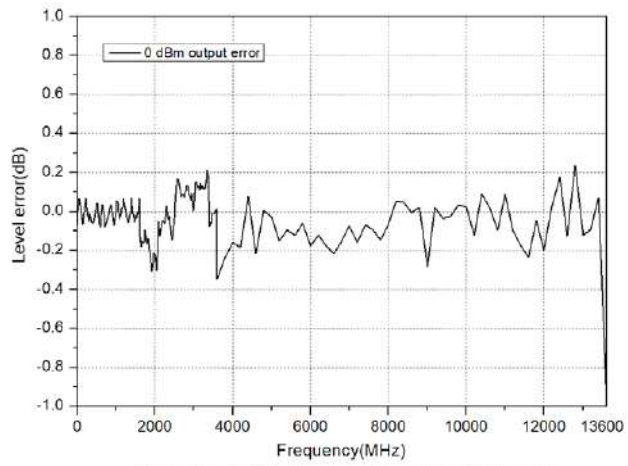
Measured at 0 dBm, level error vs frequency
