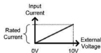
CC Mode
