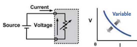
C.P Mode
