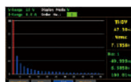
Harmonic (Bar Graph) Measurement
