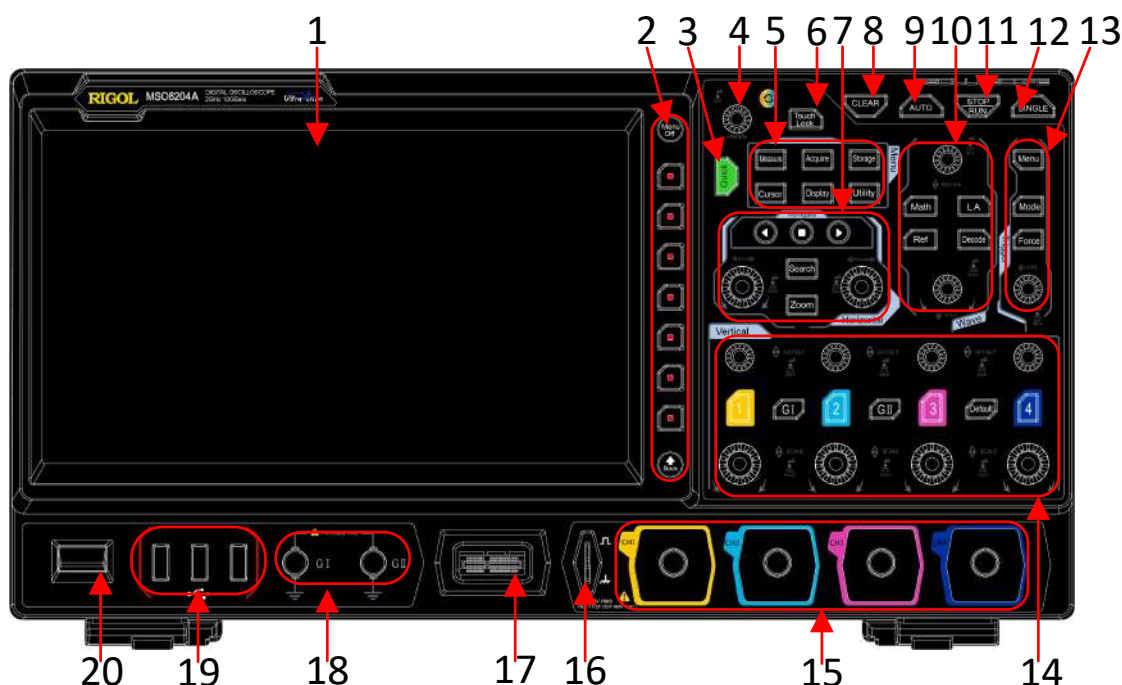
Figure 6.1 Front Panel
