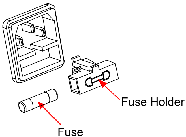
Figure 11.1 Fuse Replacement
