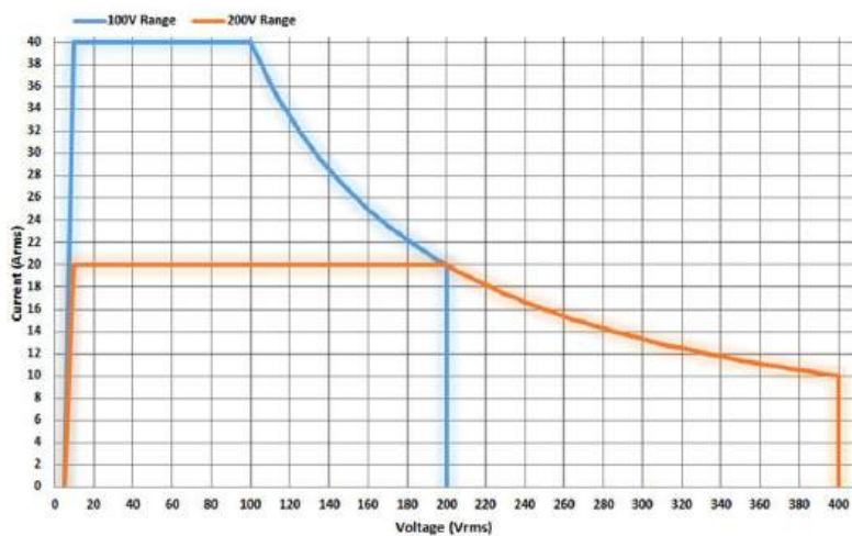
ASR-3400 and ASR-3400HF AC Mode Output Operating Area
