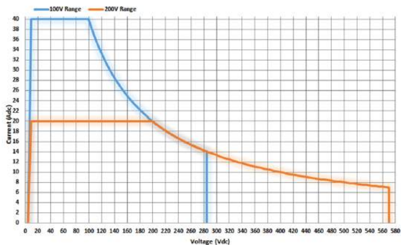
ASR-3400 and ASR-3400HF DC Mode Output Operating Area
