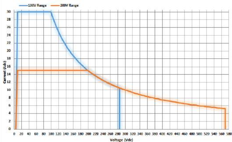
ASR-3300 DC Mode Output Operating Area
