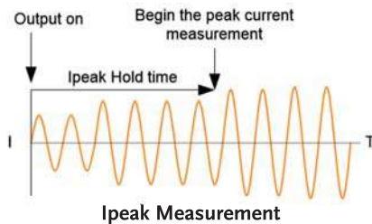
Ipeak Measurement
