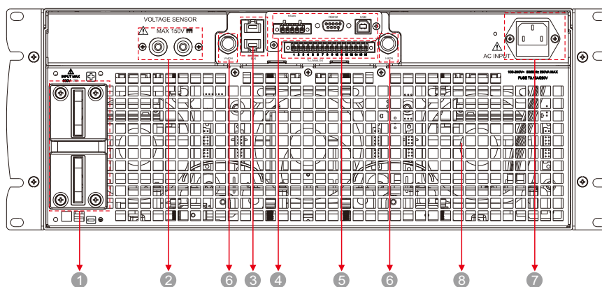
Rear Panel-4U Models as example
