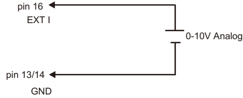
External analog input control current
